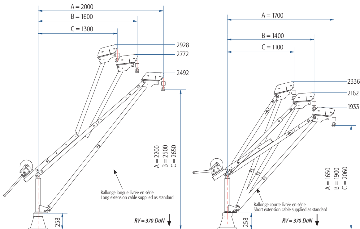
1 POTENCE = 2 MODES D'ASSEMBLAGE POSSIBLES | 1 JIB CRANE = 2 POSSIBILITIES
