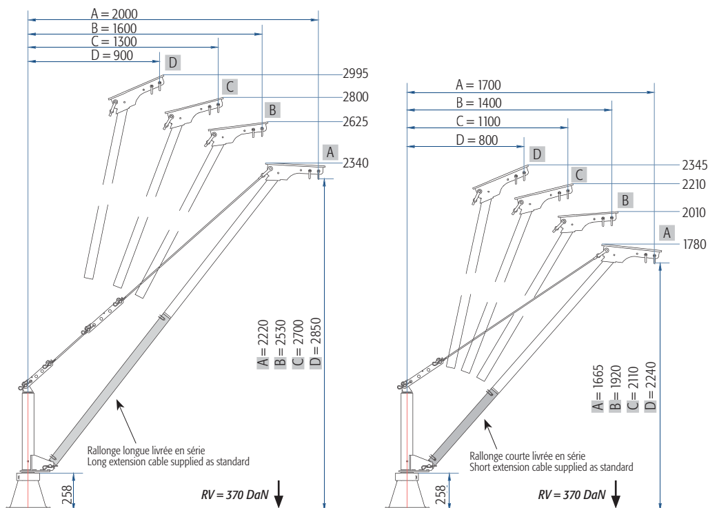
1 POTENCE = 2 MODES D'ASSEMBLAGE POSSIBLES | 1 JIB CRANE = 2 POSSIBILITIES
